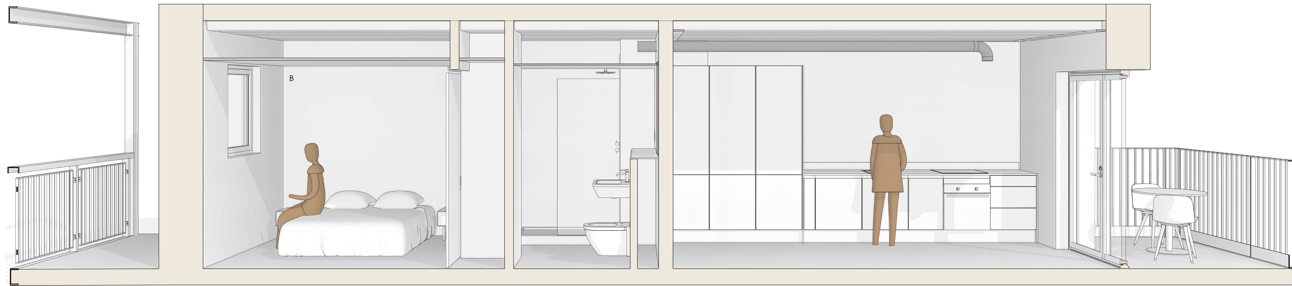
SECTION BEDROOM + LIVING 1:25
