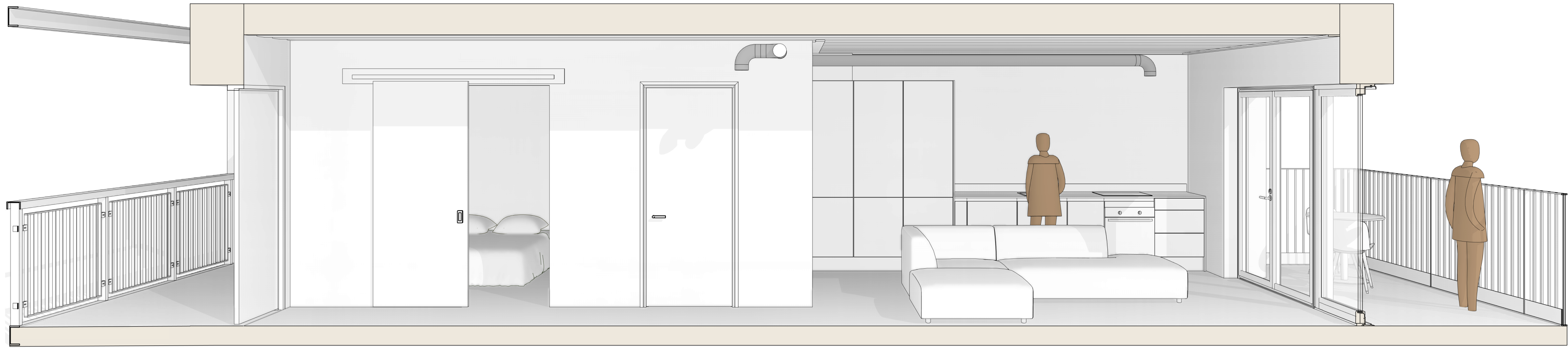
SECTION HALL + LIVING 1:25
